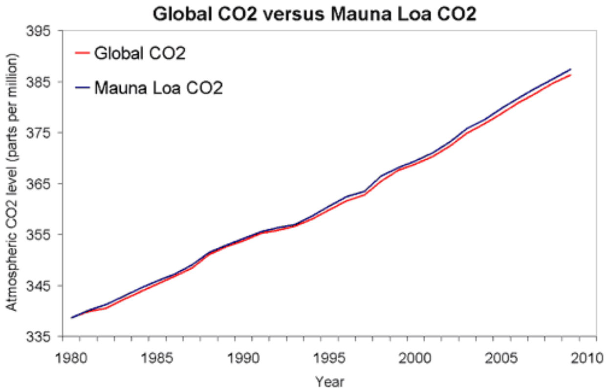
Figure 2: Global atmospheric CO2 ( NOAA ) versus Mauna Loa CO2 ( NOAA ). https://skepticalscience.com/co2-measurements-uncertainty.htm
